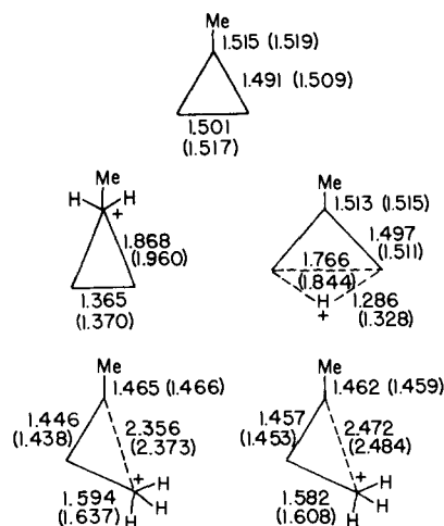
Figure 3. Structures of protonated methylcyclopropanes. The 6-31G* bond lengths are given first, followed by the 3-21G bond lengths in parentheses.
