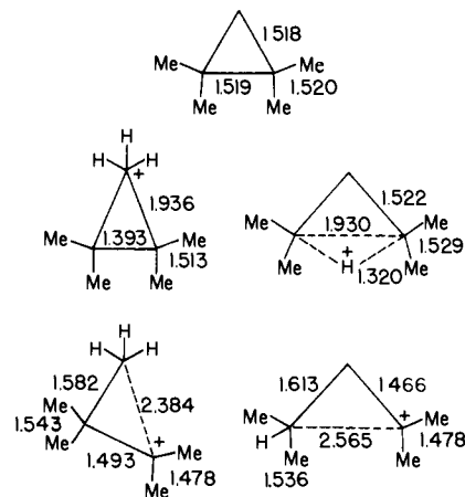
Figure 4. Structures of protonated 1,1,2,2-tetramethylcyclopropane obtained by using the 3-21G basis set.
