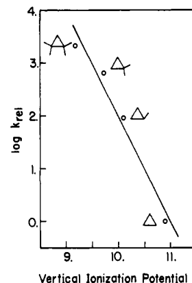
Figure 2. Correlation between \log k_{rel} and the ionization potentials for alkylcyclopropanes.
