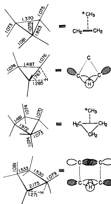
Figure 1. 6-31G optimized geometries for protonated cyclopropane and cyclobutane.
